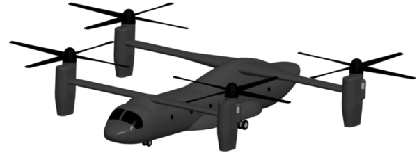
Fig. 2 Baseline quad tilt-rotor configuration (courtesy Gerardo Nunez, Aeroflightdynamics Directorate, U.S. Army).
